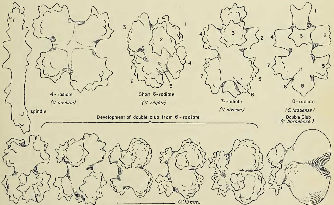
FIG. 3. Spicule types in the genus Corallium .
